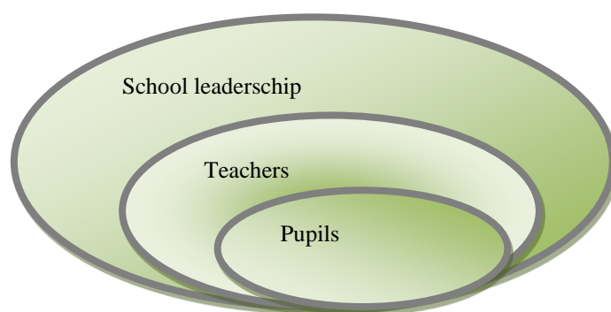
Fig.1.2. Educational ecosystem
